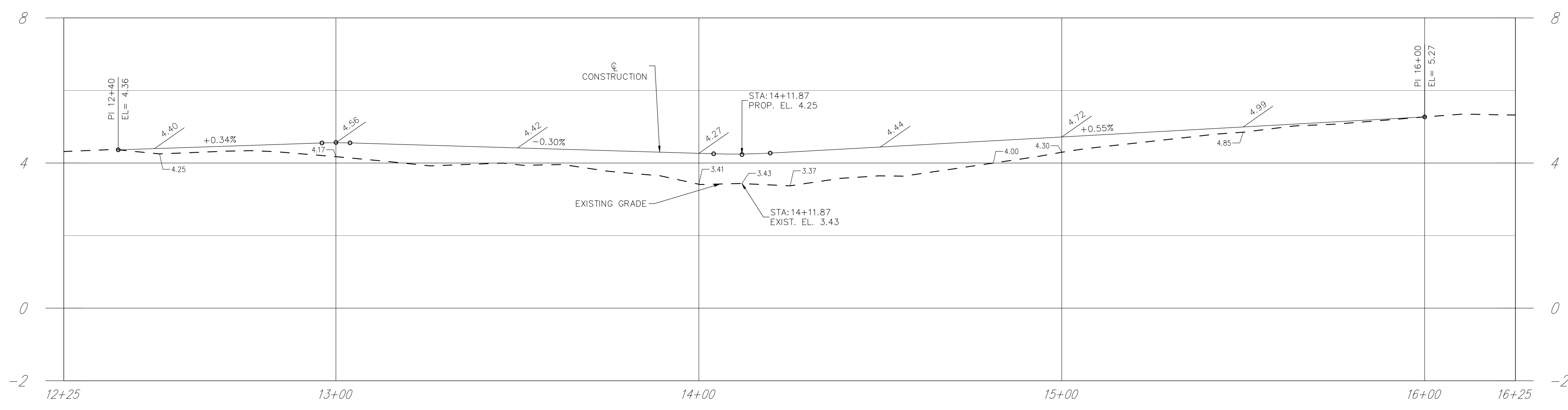
PROFILE VIEW NE 172ND STREET SCALE H 1"=20' V 1"=2'
