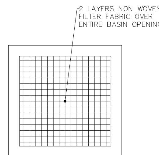
CATCH BASIN FILTER FABRIC NTS
